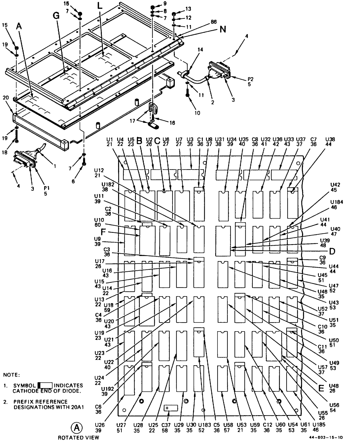
Figure 4. Electronic Component Assembly Logic No. 1 (Sheet 1 of 4)
