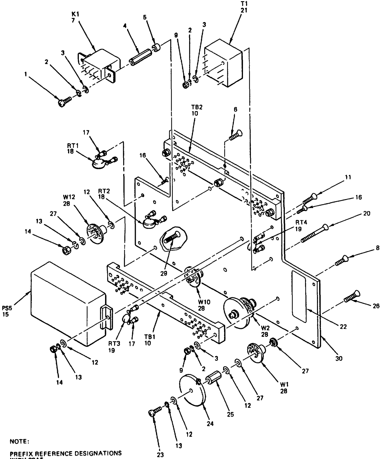
Figure 8. Signal Processor Unit Front Subassembly Exploded View
