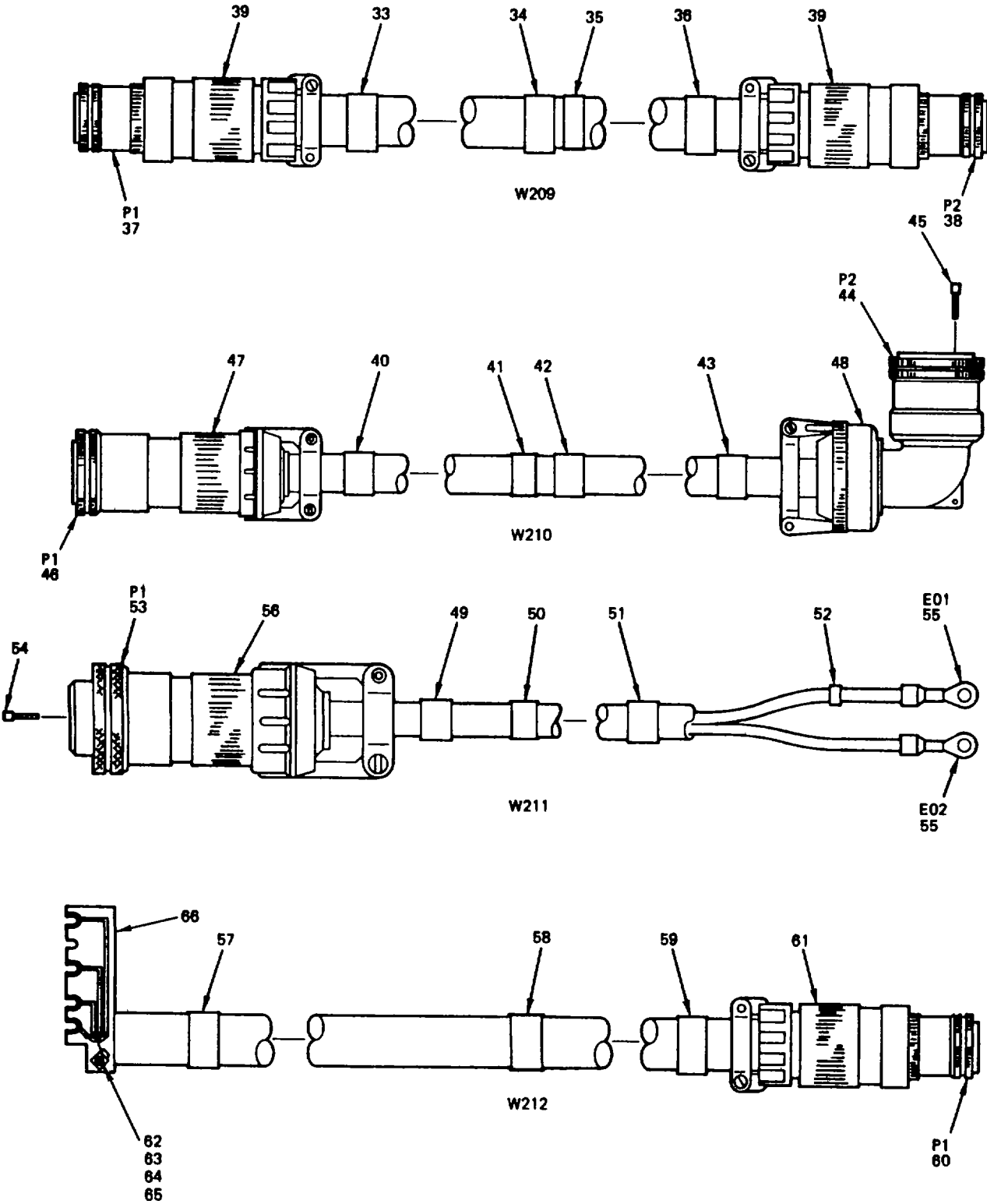
Figure 13. System Test Equipment Cable Assembly Exploded View (Sheet 2 of 2)
