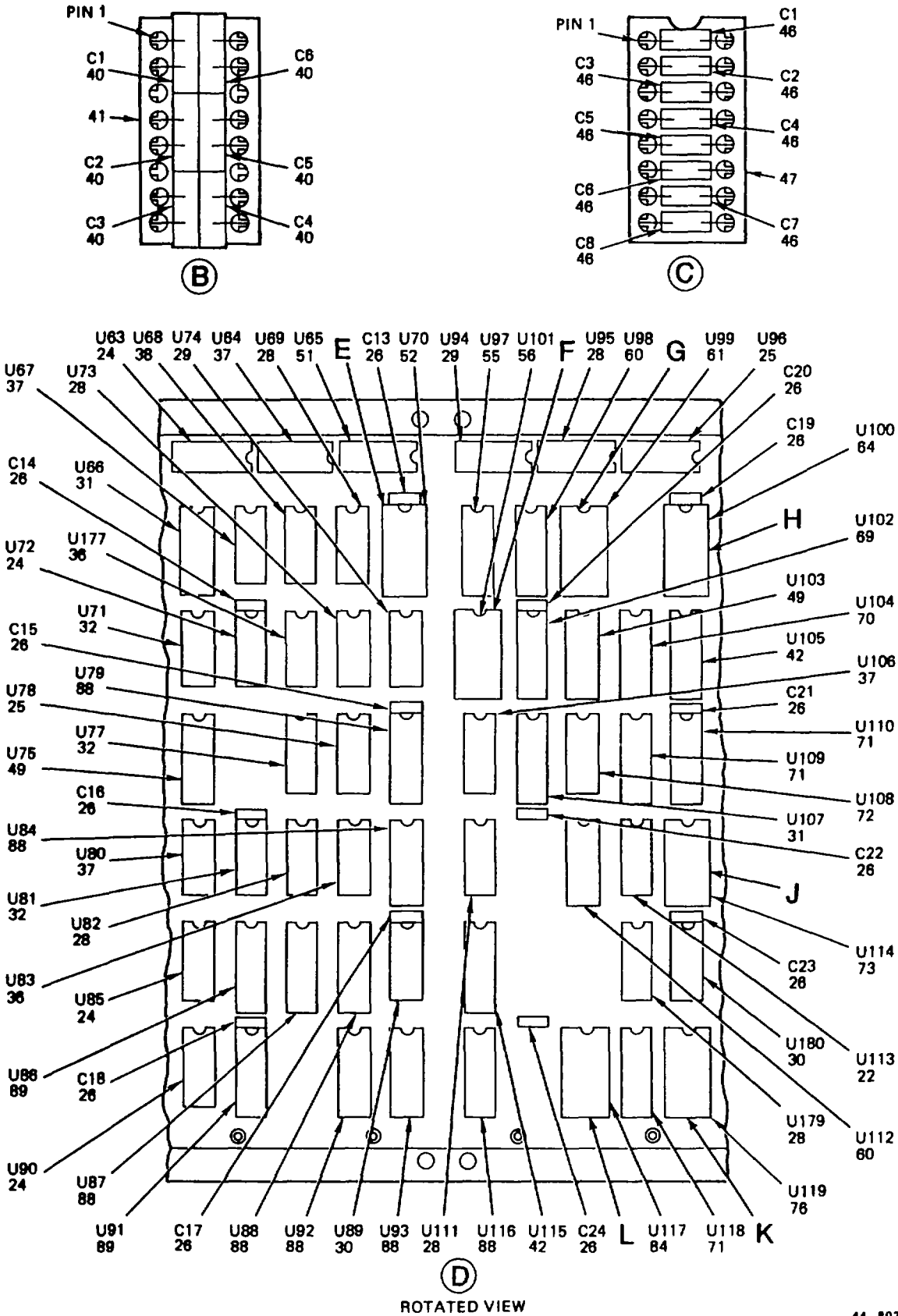
Figure 6. Electronic Component Assembly Logic No. 3 (Sheet 3 of 5)
