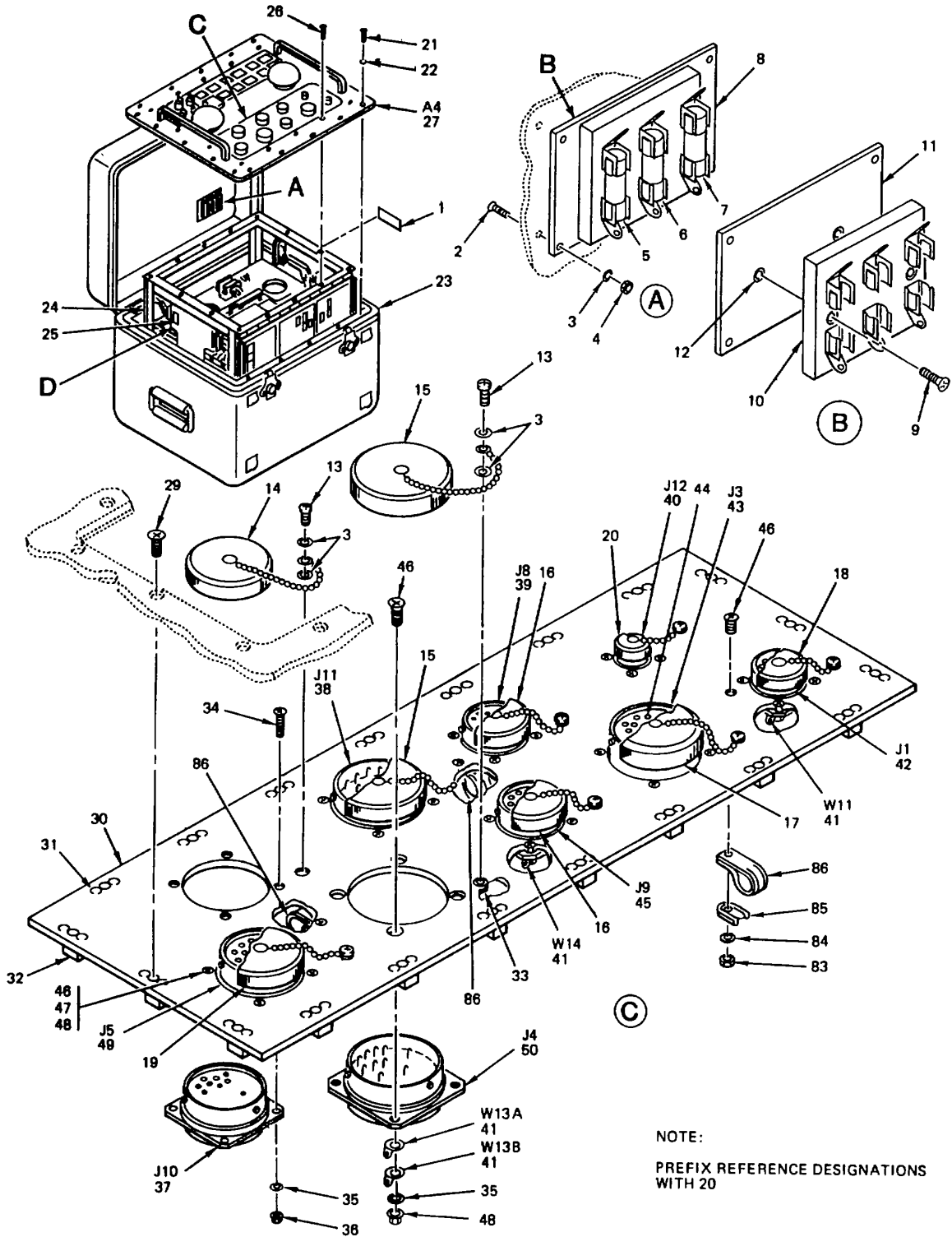
Figure 2. Signal Processor Unit Exploded View (Sheet 1 of 3)
