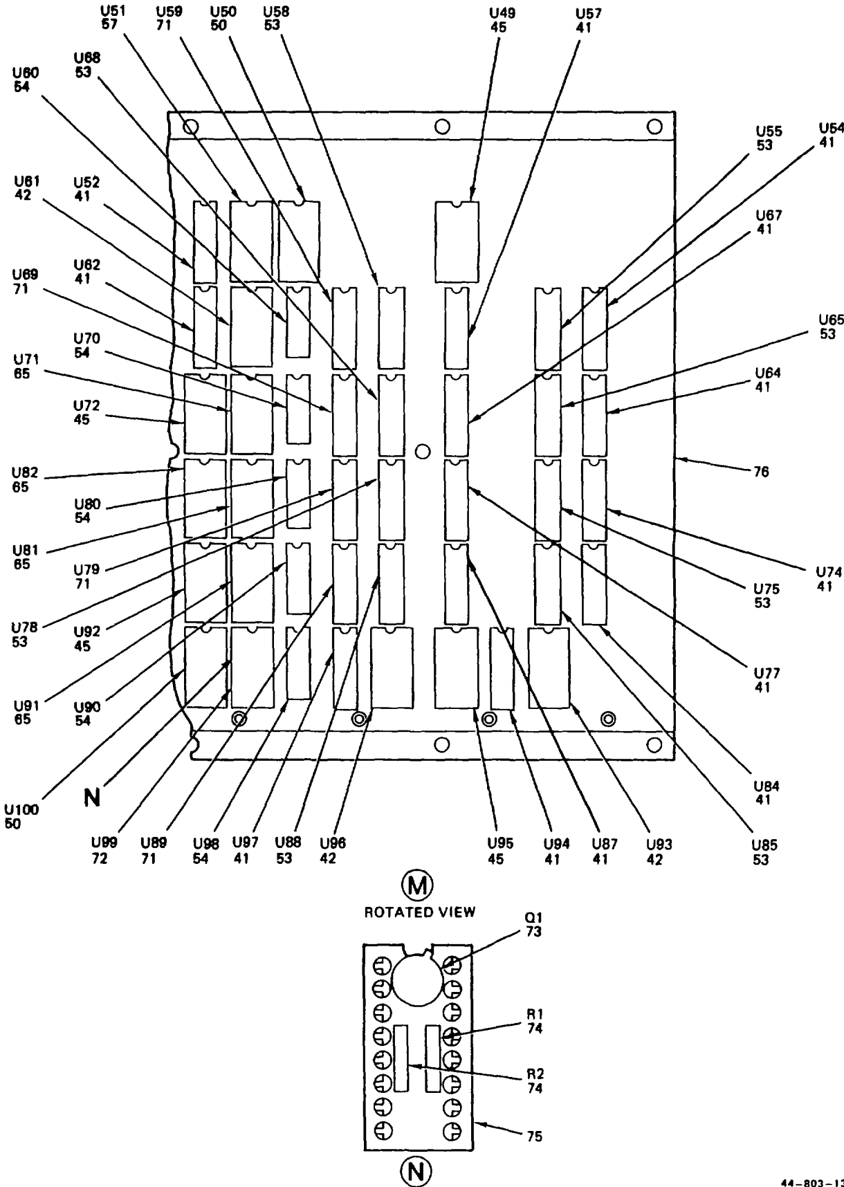
Figure 10. Buffer Box Exploded View (Sheet 4 of 4)
