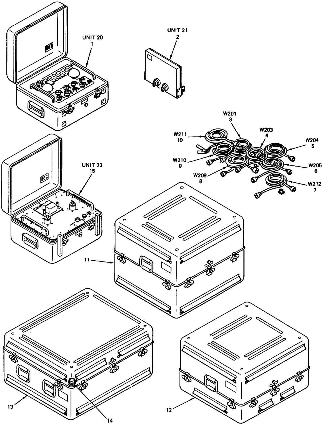
Figure 1. PADS Test Set
