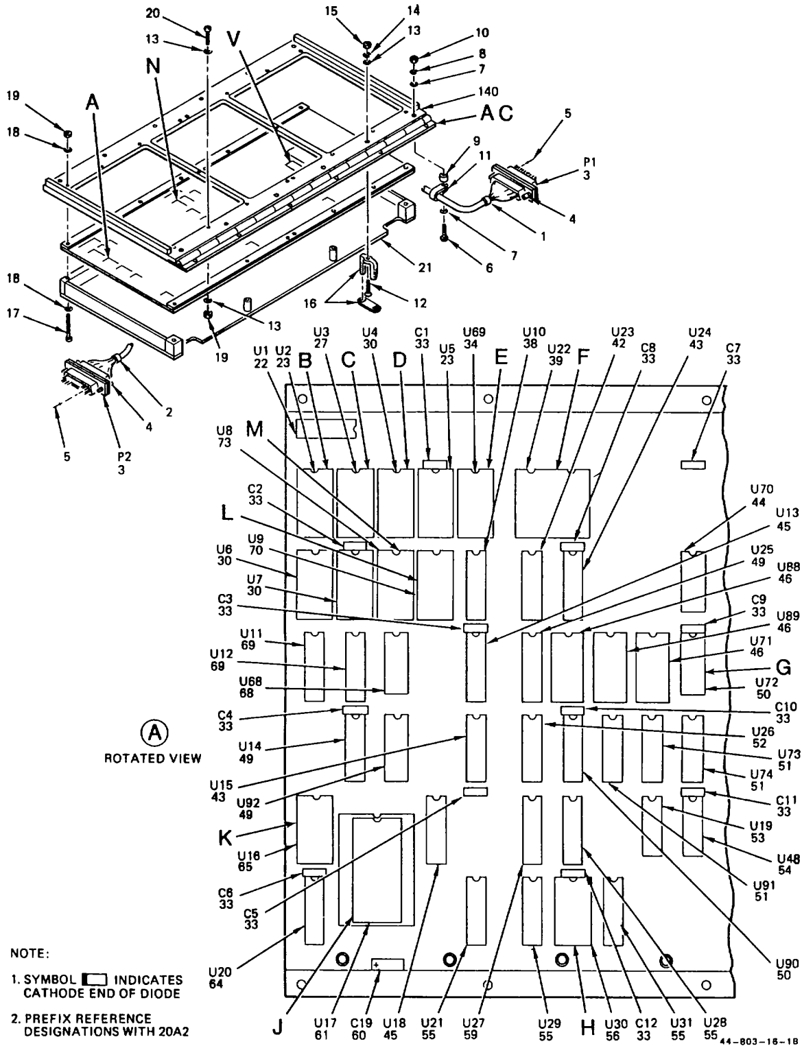
Figure 5. Electronic Component Assembly Logic No.2 (Sheet 1 of 7)
