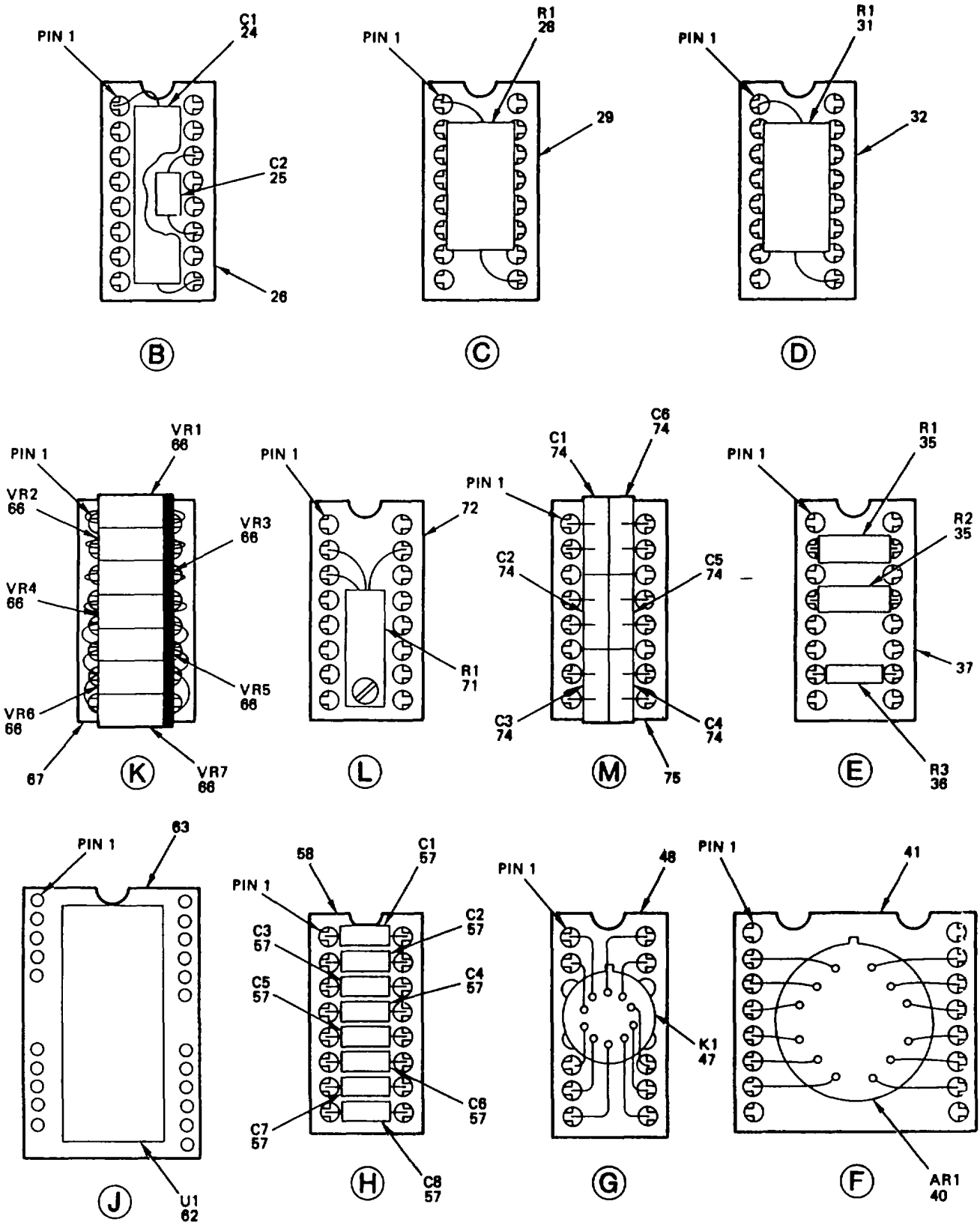
Figure 5. Electronic Component Assembly Logic No. 2 (Sheet 2 of 7)
