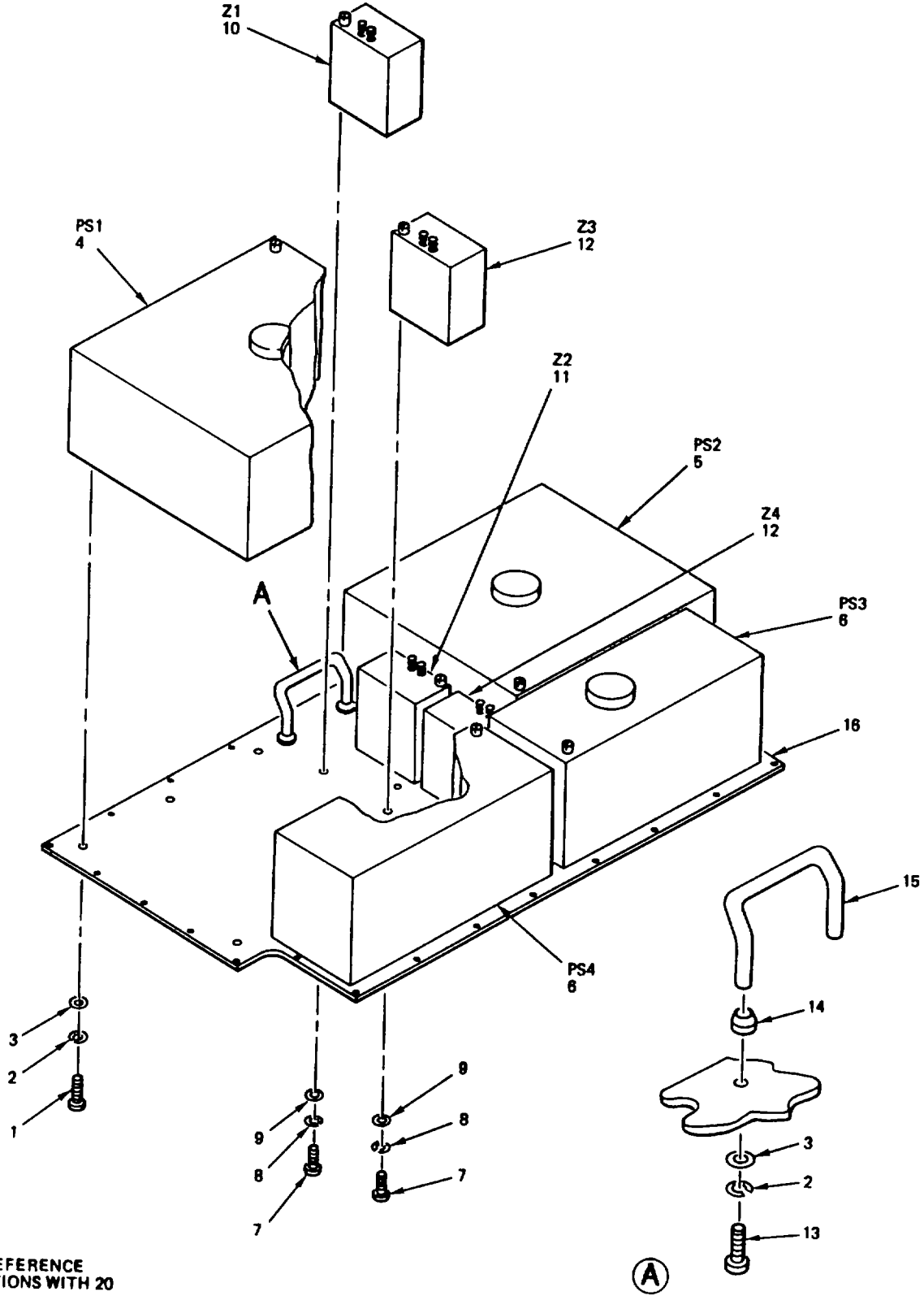
Figure 9. Signal Processor Unit Power Supply Exploded View
