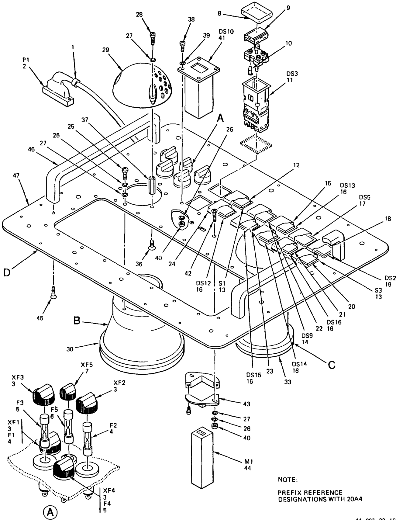
Figure 7. Signal Processor Unit Panel Assembly Exploded View (Sheet 1 of 2)
