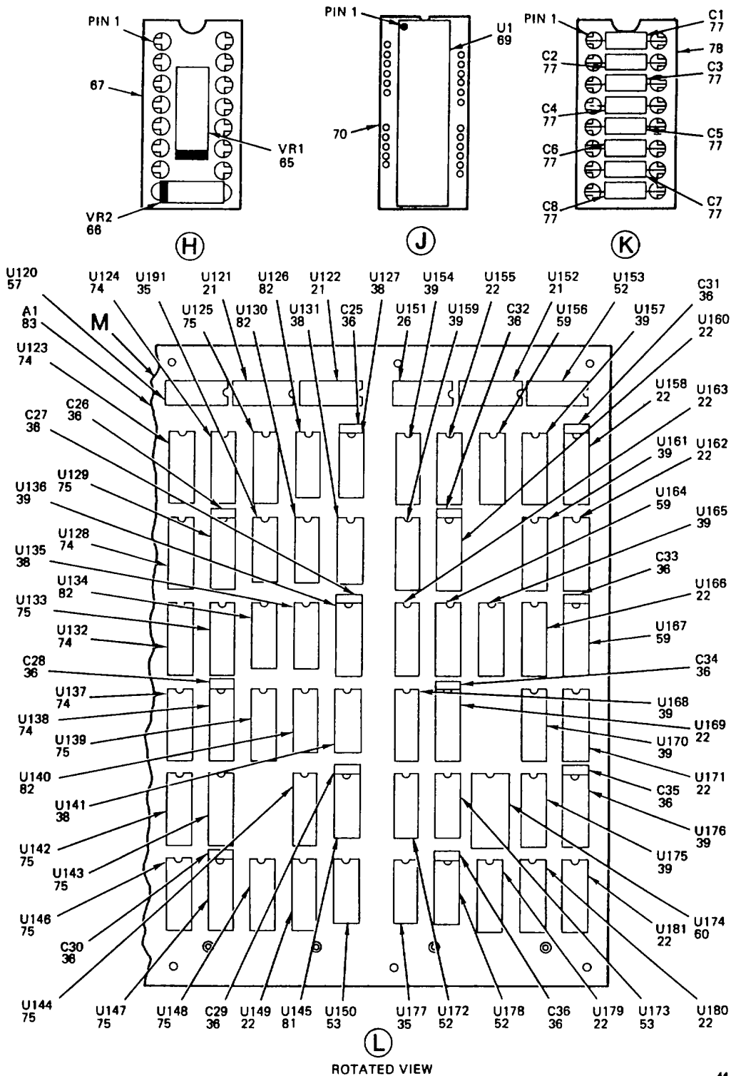
Figure 4. Electronic Component Assembly Logic No. 1 (Sheet 3 of 4)
