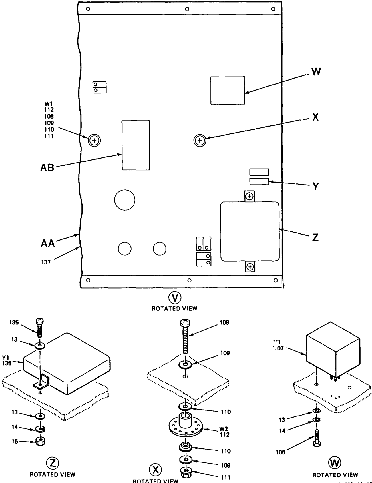
Figure 5. Electronic Component Assembly Logic No. 2 (Sheet 5 of 7)
