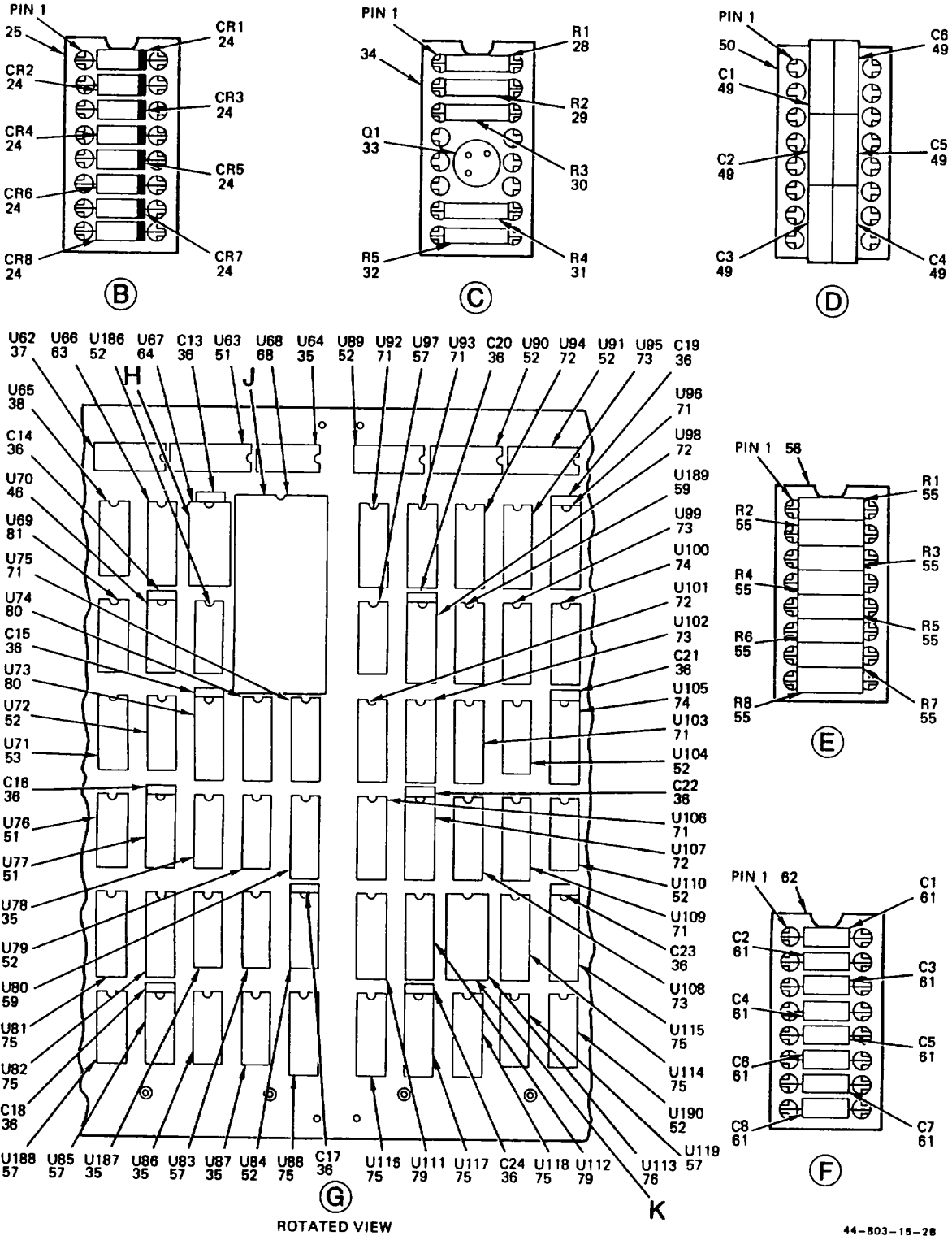
Figure 4. Electronic Component Assembly Logic No. 1 (Sheet 2 of 4)
