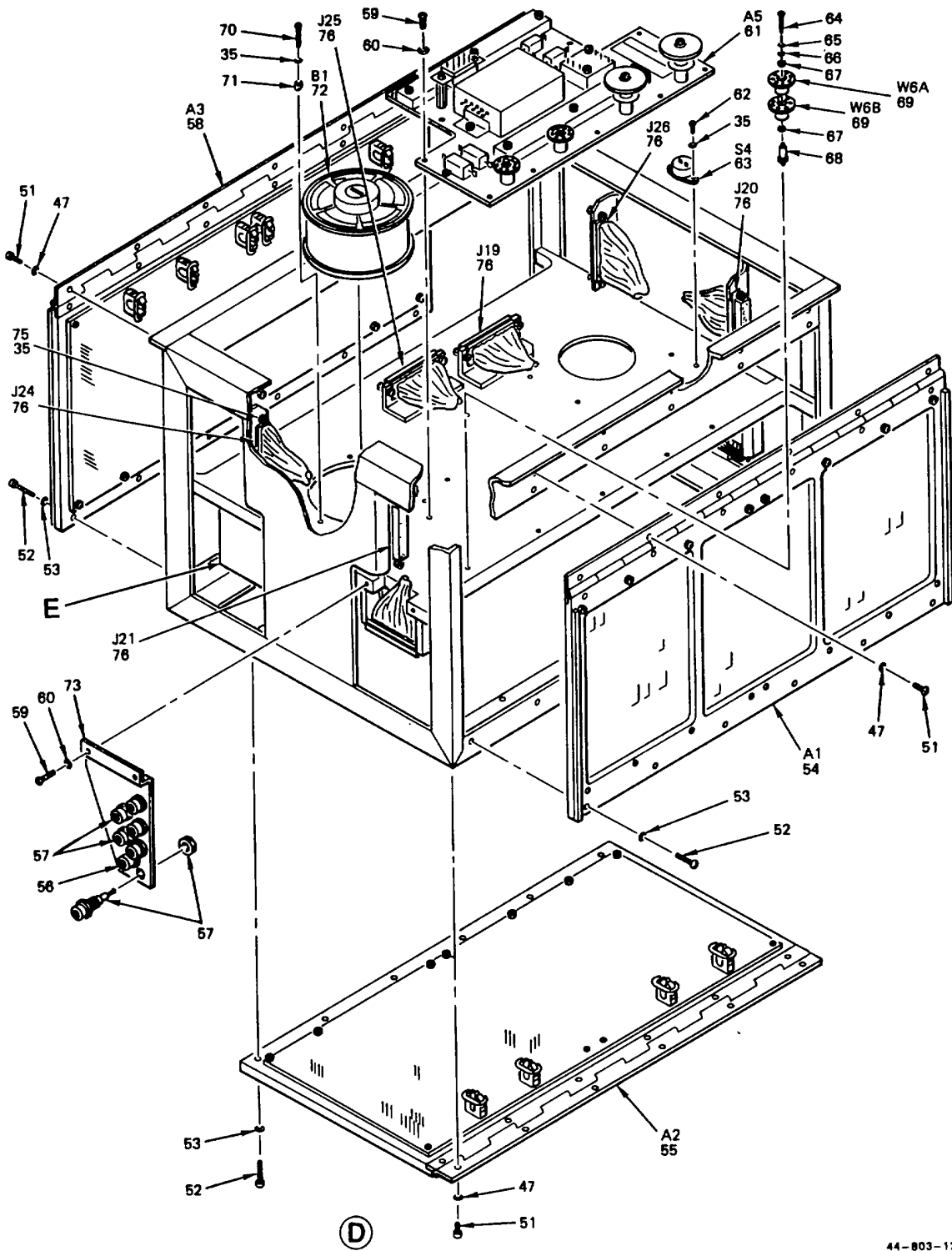
Figure 2. Signal Processor Unit Exploded View (Sheet 2 of 3)
