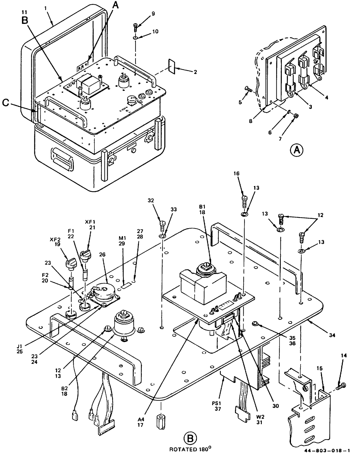
Figure 11. Punched Tape Reader (Sheet 1 of 2)
