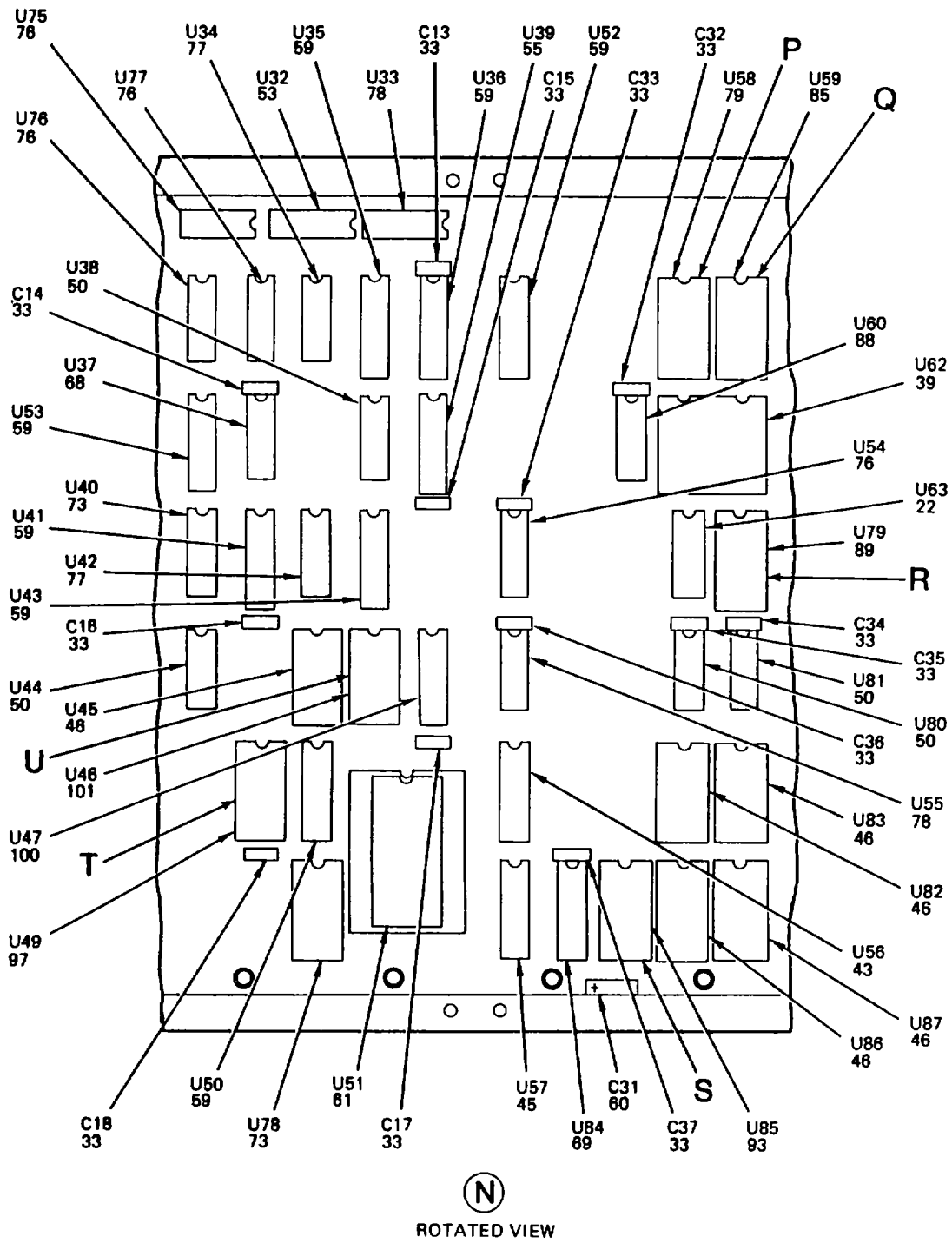
Figure 5. Electronic Component Assembly Logic No. 2 (Sheet 3 of 7)
