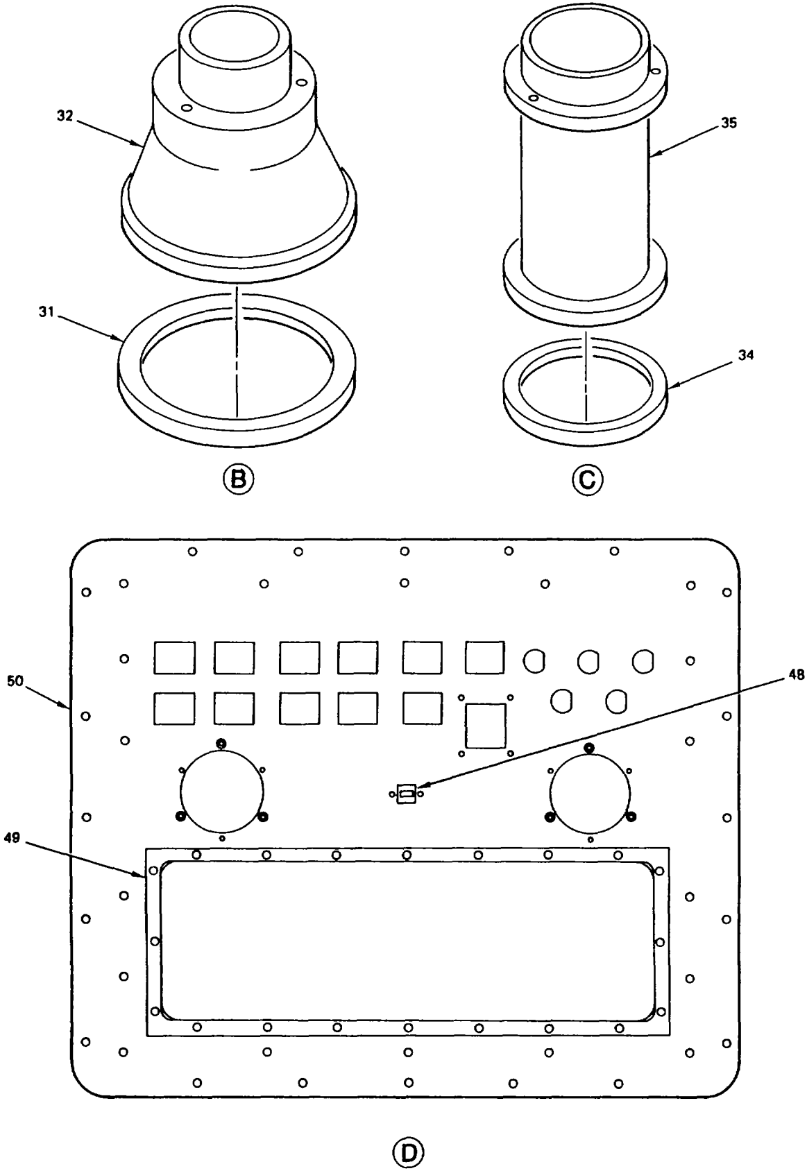
Figure 7. Signal Processor Unit Panel Assembly Exploded View (Sheet 2 of 2)
