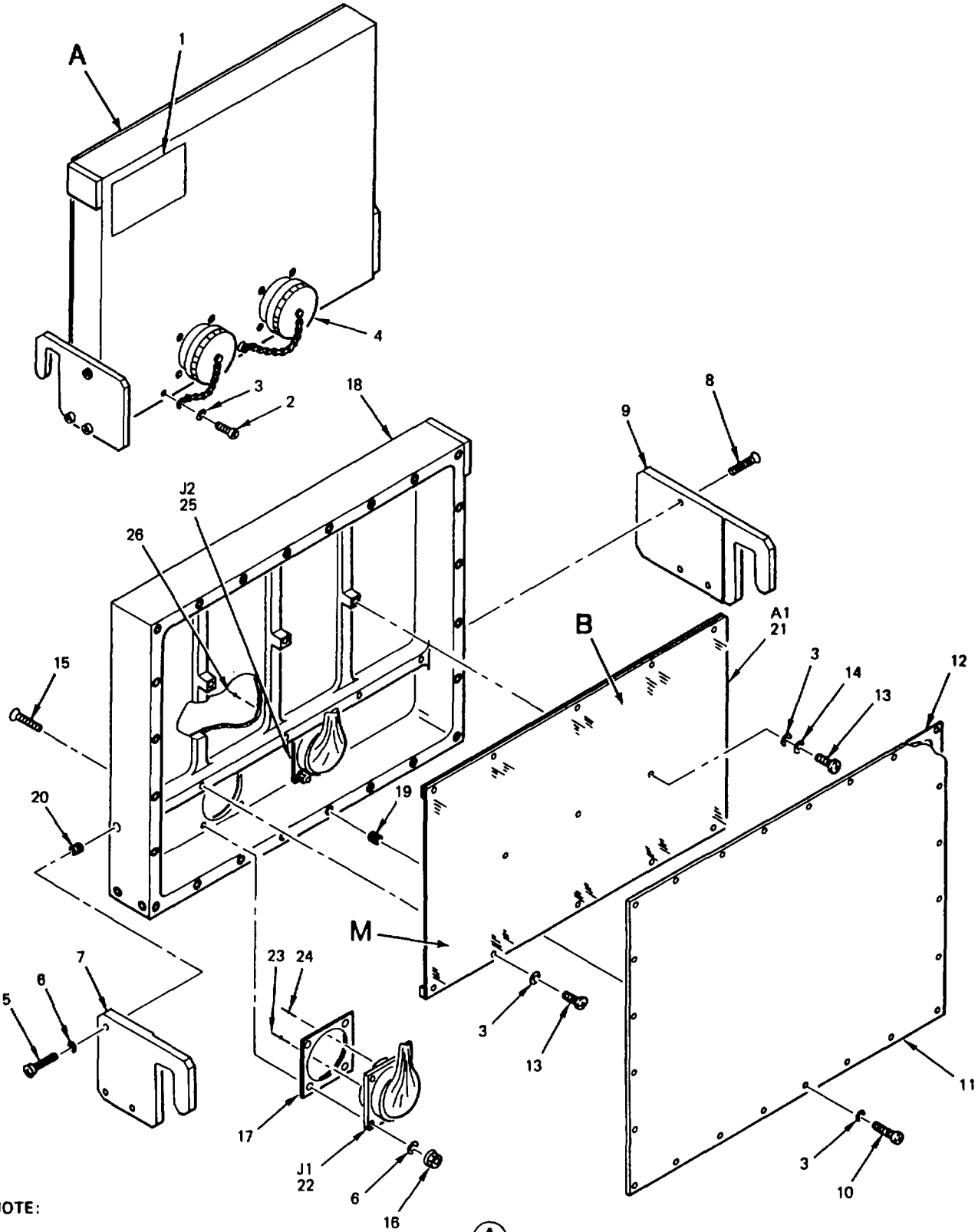
Figure 10. Buffer Box Exploded View (Sheet 1 of 4)
